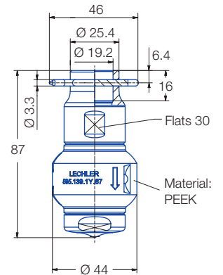
Dimensions slip-on connection according to ASME-BPE (OD-tube) 595.139.1Y.67
