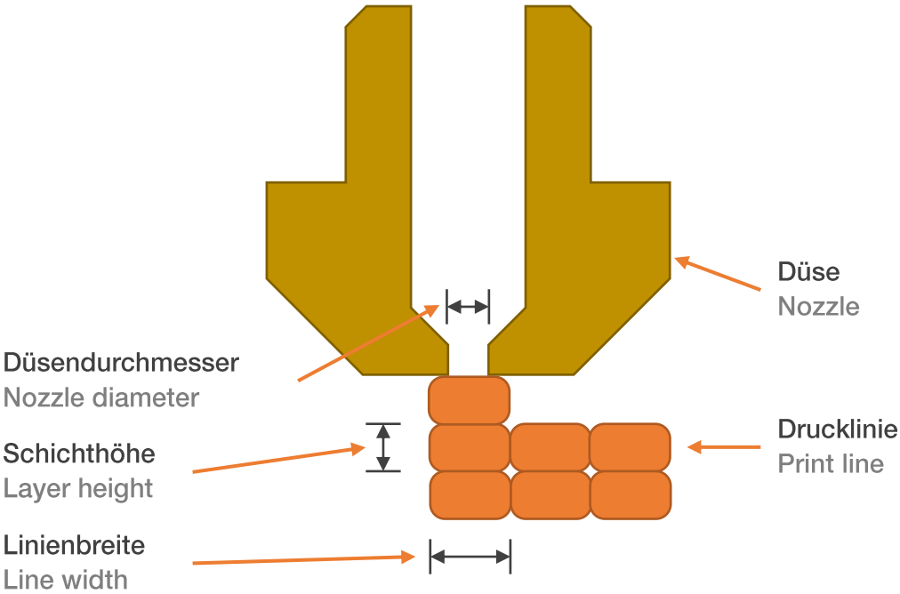
1: Schema Filament-3D-Drucker – Filament 3D printer schematic
